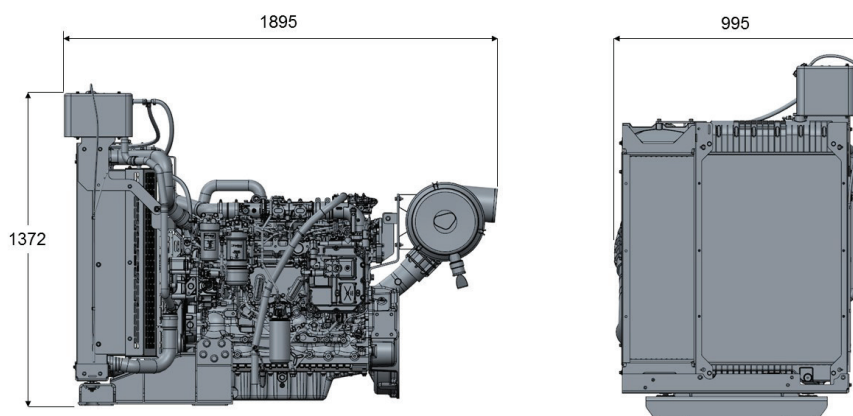
Engine package weights and dimensions
